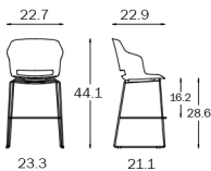
STOOL WITH SLED FRAME
