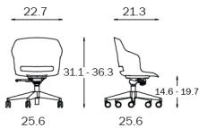
5 STAR BASE WITH KNEE TILT
