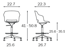
TECHNICAL STOOL
