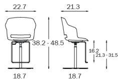
STOOL WITH GAS LIFT
