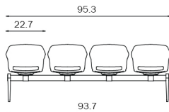
4 SEATER BENCH
